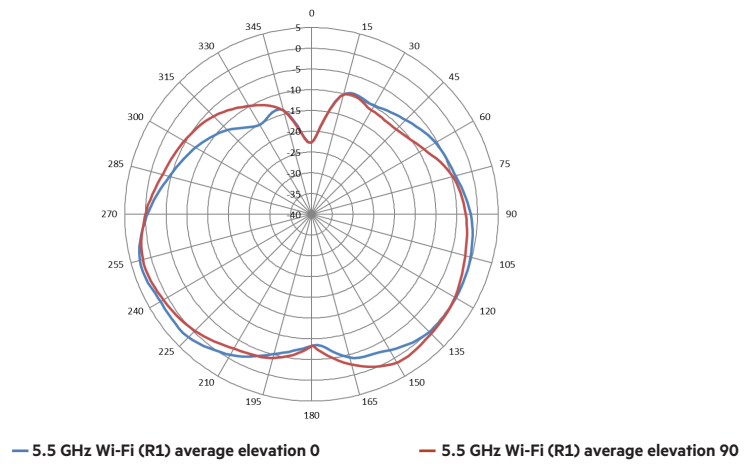
Figure 5. 5.5 GHz Wi-Fi antenna patterns (vertical)
