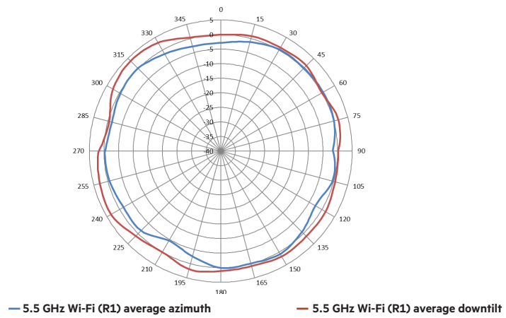
Figure 2. 5.5 GHz Wi-Fi antenna patterns (horizontal)
