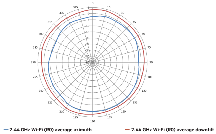
Figure 1. 2.44 GHz Wi-Fi antenna patterns (horizontal)
