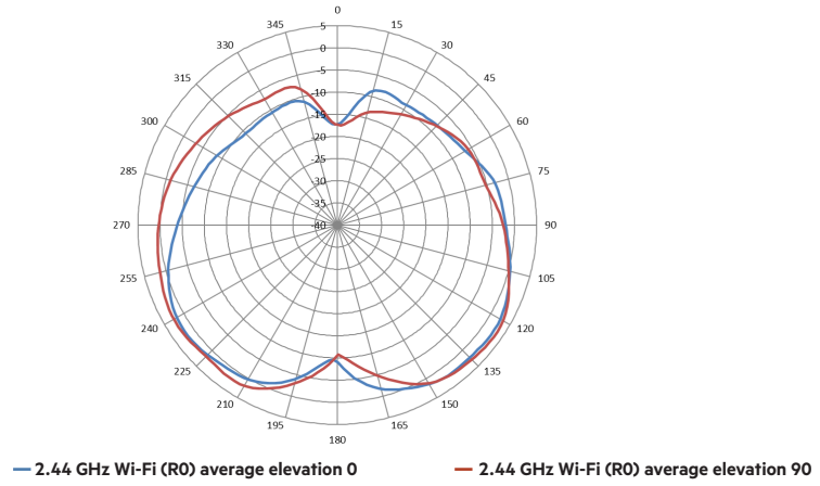
Figure 4. 2.44 GHz Wi-Fi antennas patterns (vertical)
