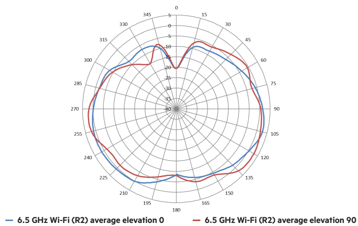
Figure 6. 6.5 GHz Wi-Fi antennas patterns (vertical)
