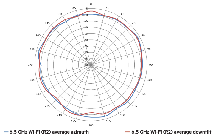
Figure 3. 6.5 GHz Wi-Fi antenna patterns (horizontal)
